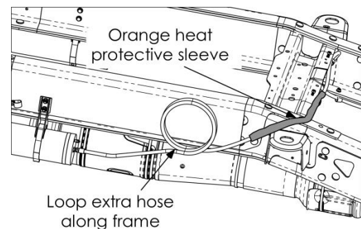
Figure 43. Location of extra hose on passenger side.
