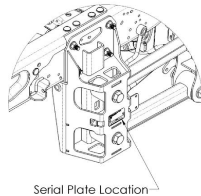
Figure 2. Serial Number Tag Location
