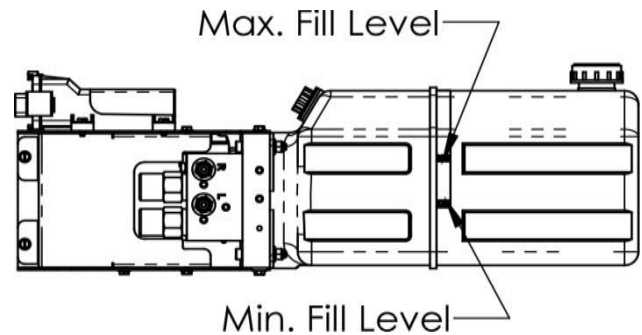
Figure 67. Final fill fluid level.
