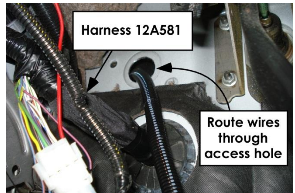
Figure 53. External Harness routing through firewall.
