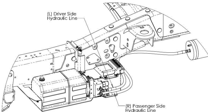
Figure 40. Power Module hose attachment.
