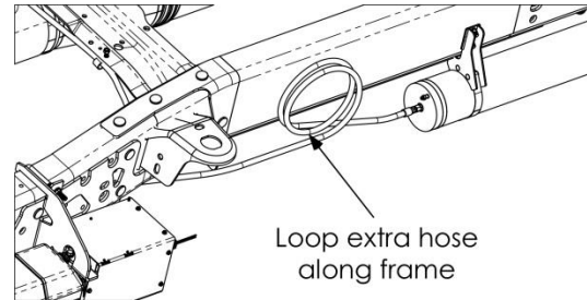
Figure 41. Location of extra hose on driver side.
