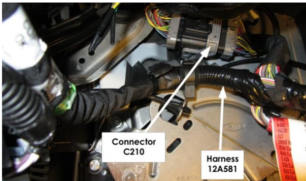
Figure 62. Wiring bundle to access (Diesel shown).
