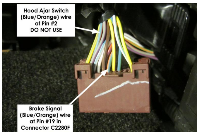
Figure 66. Wire to splice in Connector C2280F.
