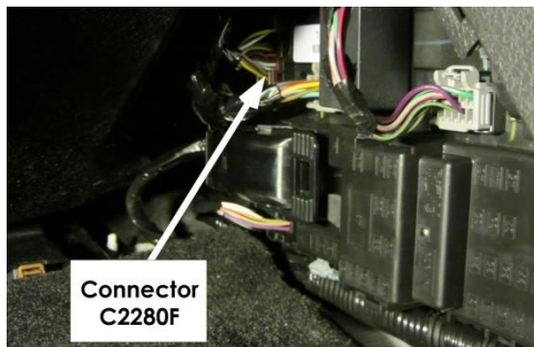
Figure 65. Location of Connector C2280F.
