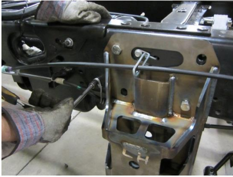
Figure 50. Attachment of wire formed bracket.
