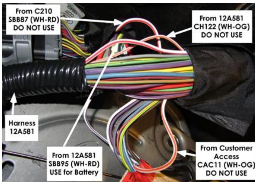
Figure 63. Identification of wire to splice.
