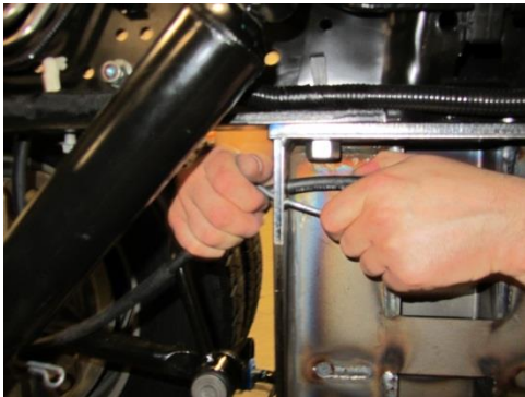
Figure 45. Feeding parking brake cable, and wire formed bracket, through hanger.
