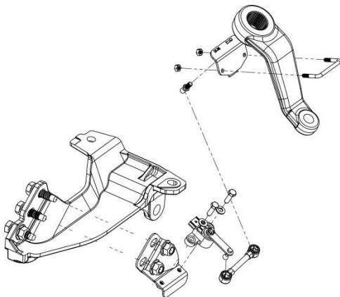
Figure 55. Steering Sensor Installation.
