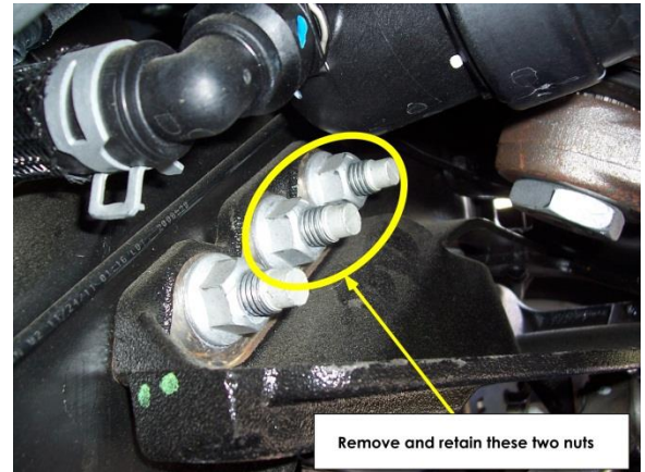
Figure 56. Track rod mount bolts to temporarily remove.
