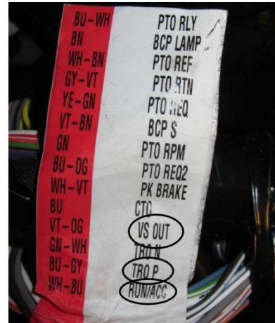
Figure 61. Customer access wires utilized.
