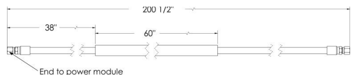
Figure 42. [DS147F Only] Orientation of passenger side -4 hose.
