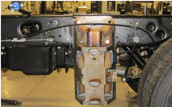
Figure 52. Complete driver side parking brake cable re-routing.
