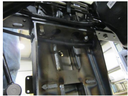
Figure 48. Grommets and parking brake cable after installation through hanger.
