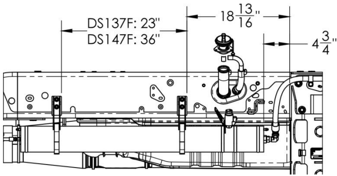
Figure 36. Secondary Volume suggested mount locations
