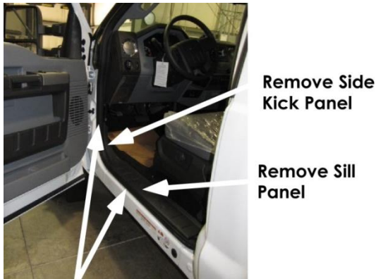
Figure 58. Accessing inside of side kick panel.
