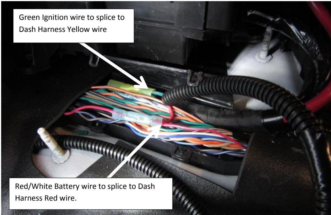
Figure 58 Green and Red/White wires spliced to Dash Harness
