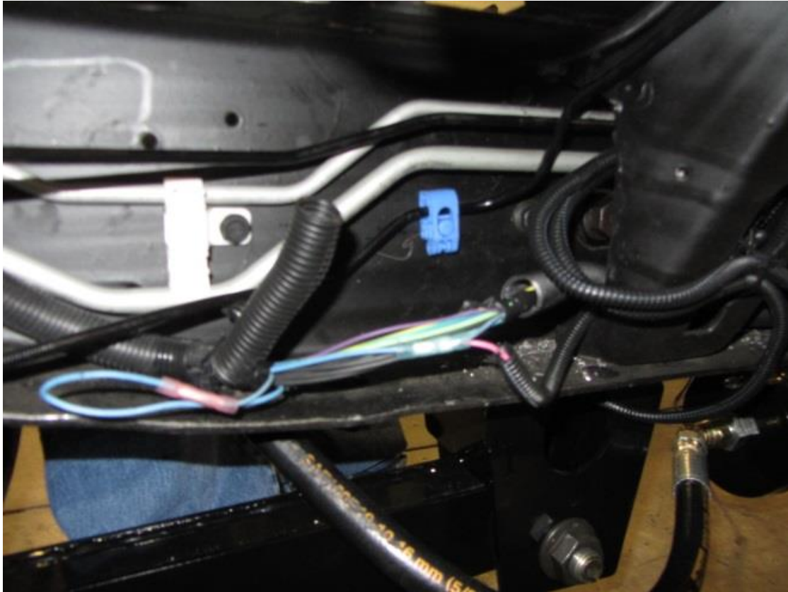
Figure 63. OEM Light Blue (Brake) wire spliced to LiquidSpring Pink/Black wire.
